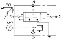
HİDROLİK SEMBOL HYDRAULIC SYMBOL
